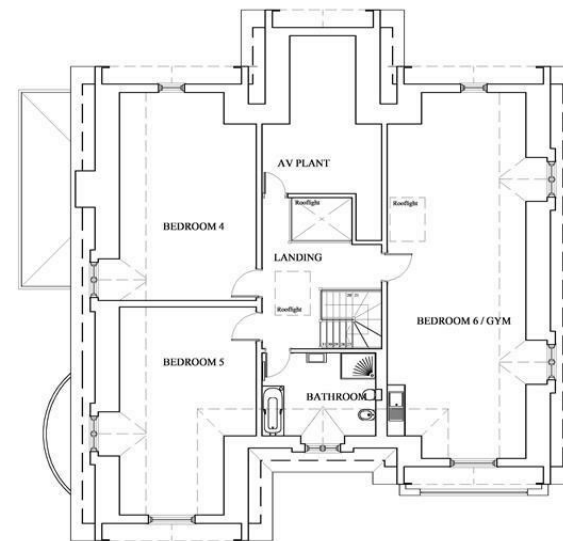
G SECOND FLOOR PLAN
